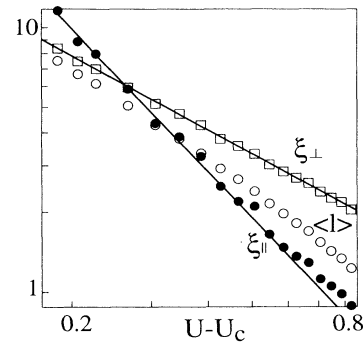
FIG. 3. Monte Carlo results for q=1.0 and K_2=0.1 . Shown are data for the roughness (open squares), the parallel correlation length (closed circles), and the mean separation \langle l \rangle (open circles).
