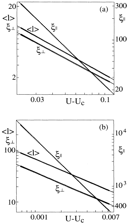
FIG. 2. (a) Transfer-matrix results for K_2=\infty and K_1=K_3 ( q=0 and \theta=\pi/2 ). Data for the parallel correlation length \xi_{\parallel} , the mean separation \langle l \rangle , and the roughness \xi_{\perp} are shown as a function of the potential depth U . (b) Results for K_1/K_2=K_3/K_2=31.5 .
