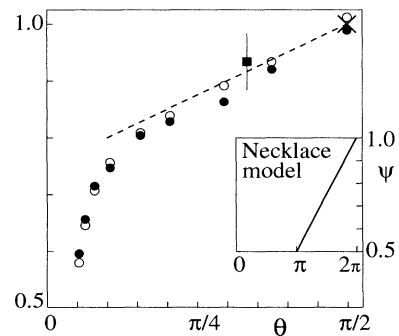
FIG. 4. Results for the exponents \psi (open symbols) and \nu_{\perp} (filled symbols). The square denotes the Monte Carlo result for \nu_{\perp} , the circles denote transfer-matrix results. In the latter case, the error bars are the size of the symbols. The cross denotes the exactly known result for the case \theta=\pi/2 , namely \psi=\nu_{\perp}=1 . The inset shows the results for the necklace model, with discontinuous transitions for \theta < \pi .
